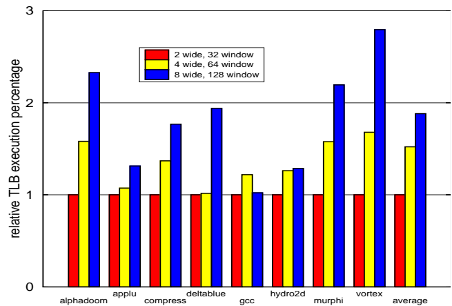
Figure 3. Overhead of software TLB miss handling as a function of superscalar width. Wider machines spend larger percentage of their execution time on TLB miss handling because TLB miss handling does not benefit much from increased issue width.
