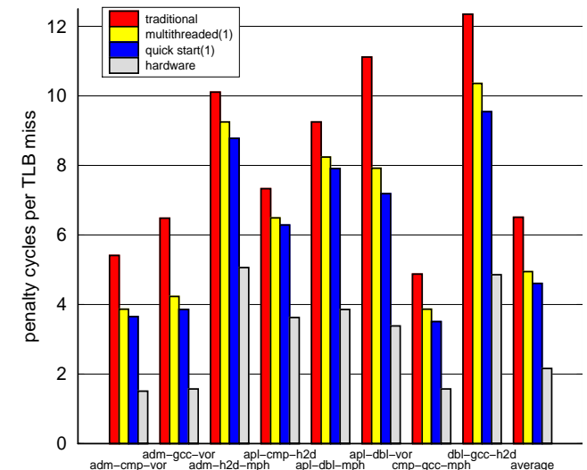
Figure 7. Average TLB miss penalties with 3 applications running on the SMT.
