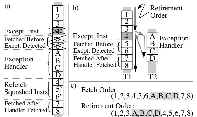
Figure 1. Traditional vs. Multithreaded Exception Handling. Six instructions have been fetched when an exception is detected on the fourth. Traditionally (a), instructions 4-6 are squashed and must be refetched after the exception handler is fetched. With our multithreaded mechanism (b), a second thread fetches the exception handler (A-D), and then the main thread continues to fetch (7,8). The exception handler is retired before the excepting instruction. (c) This makes the global retirement order different than the fetch order, but each thread retires instructions in its fetch order.
