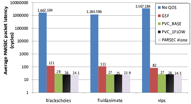
Figure 8: PARSEC results
