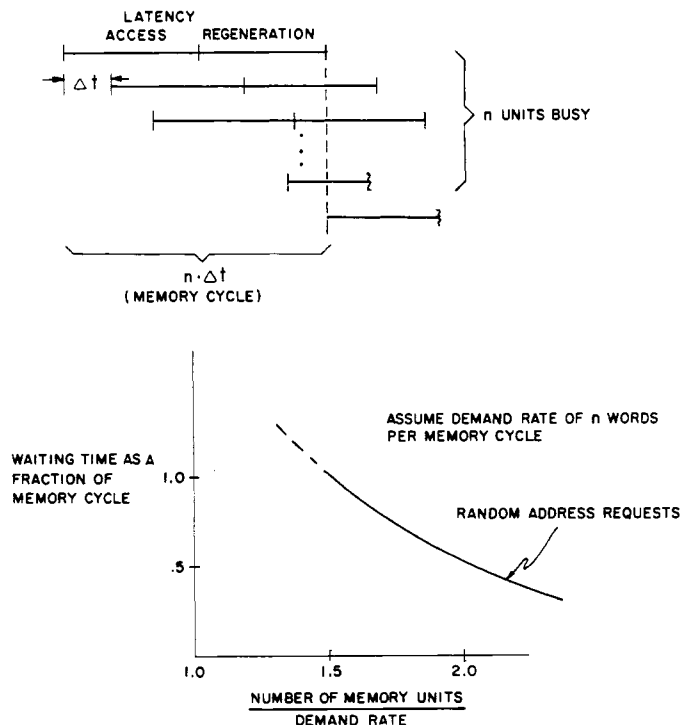
Fig. 3. Interleaving memory units.
