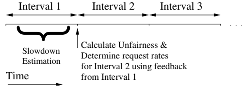
Figure 3: FST’s interval-based estimation and throttling
