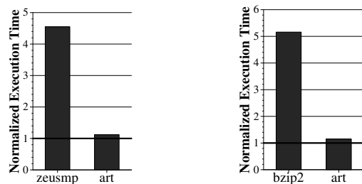
Figure 1: Disparity in slowdowns due to unfairness
