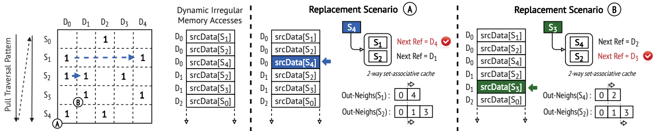
Fig. 3: Using a graph's transpose to emulate OPT: For the sake of simplicity, we assume that only irregular accesses (srcData for a pull execution) enter the 2-way cache. In a pull execution using CSC, fast access to outgoing-neighbors (i.e. rows of adjacency matrix) encoded in the transpose (CSR) enables efficient emulation of OPT.
