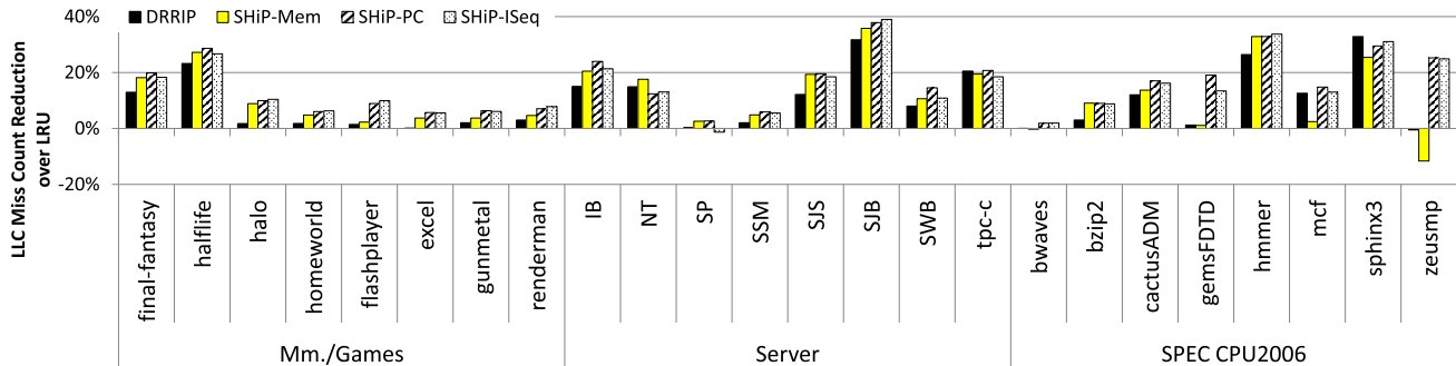
Figure 6: SHiP miss count reduction over LRU.
