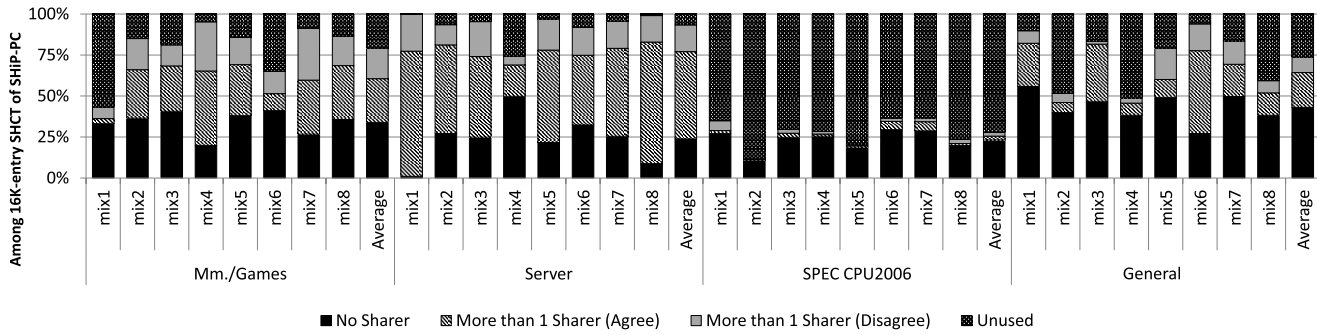
Figure 13: Utilization and aliasing for the shared 16K-entry SHCT under SHiP-PC.
