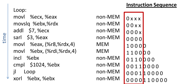
Figure 3: Example of Encoding Instruction Sequence History
