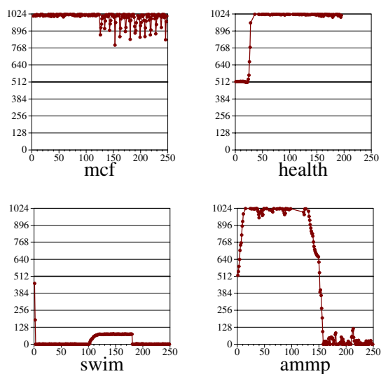
Figure 12: PSEL value during benchmark execution (horizontal axis denotes the number of instruction in Millions)
