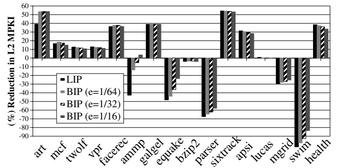
Figure 8: Comparison of Static Insertion Policies
