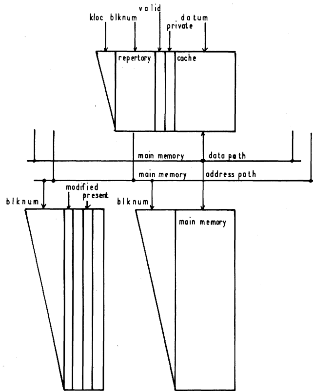
Fig. 1. Conceptual design of a multicache system.
