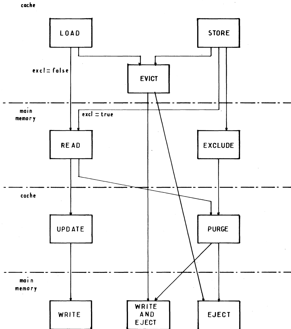
Fig. 2. Structural chart of the coherence algorithm.
