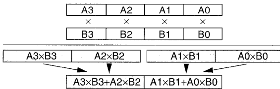
Figure 2. Packed multiply-add word to doubleword.
