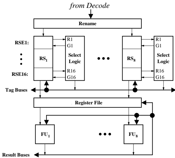
Figure 3. Processor Microarchitecture
