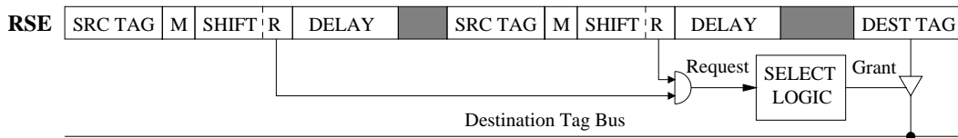
Figure 5. Scheduling Logic for One Reservation Station Entry
