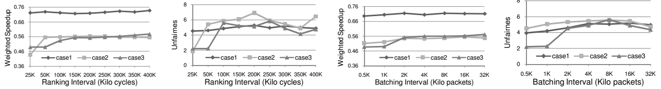
Figure 12: Effect of Ranking and Batching Intervals
