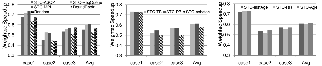
Figure 10: Performance impact of different (a) Ranking Heuristics (b) Batching Policies (c) Local Arbitration Policies
