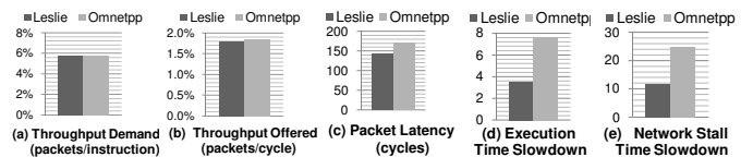
Figure 1: Different Metrics for Network Performance Analysis
