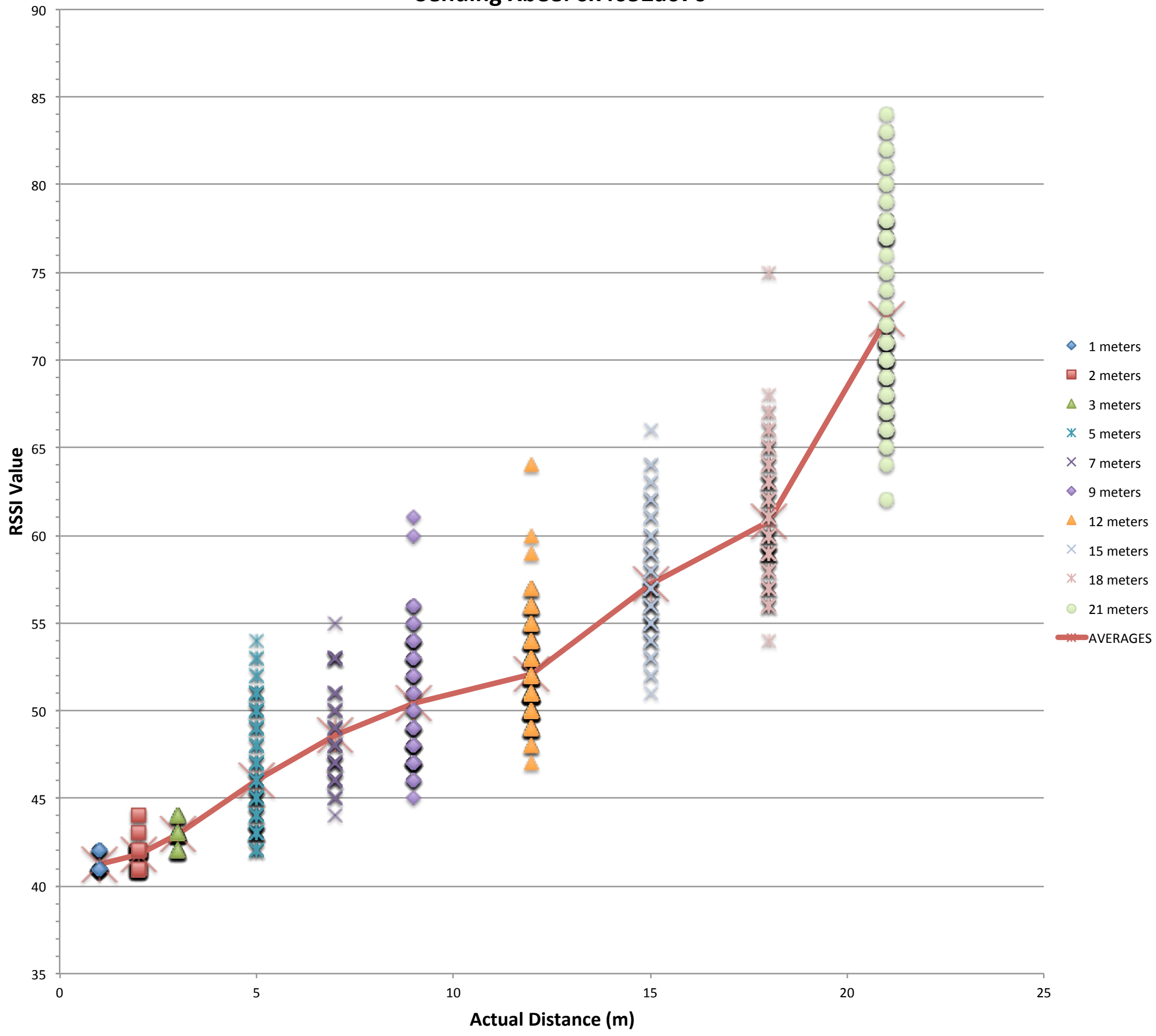
RSSI Values (Decimal) as a Function of Distance Sending Xbee: 0x4052a076
