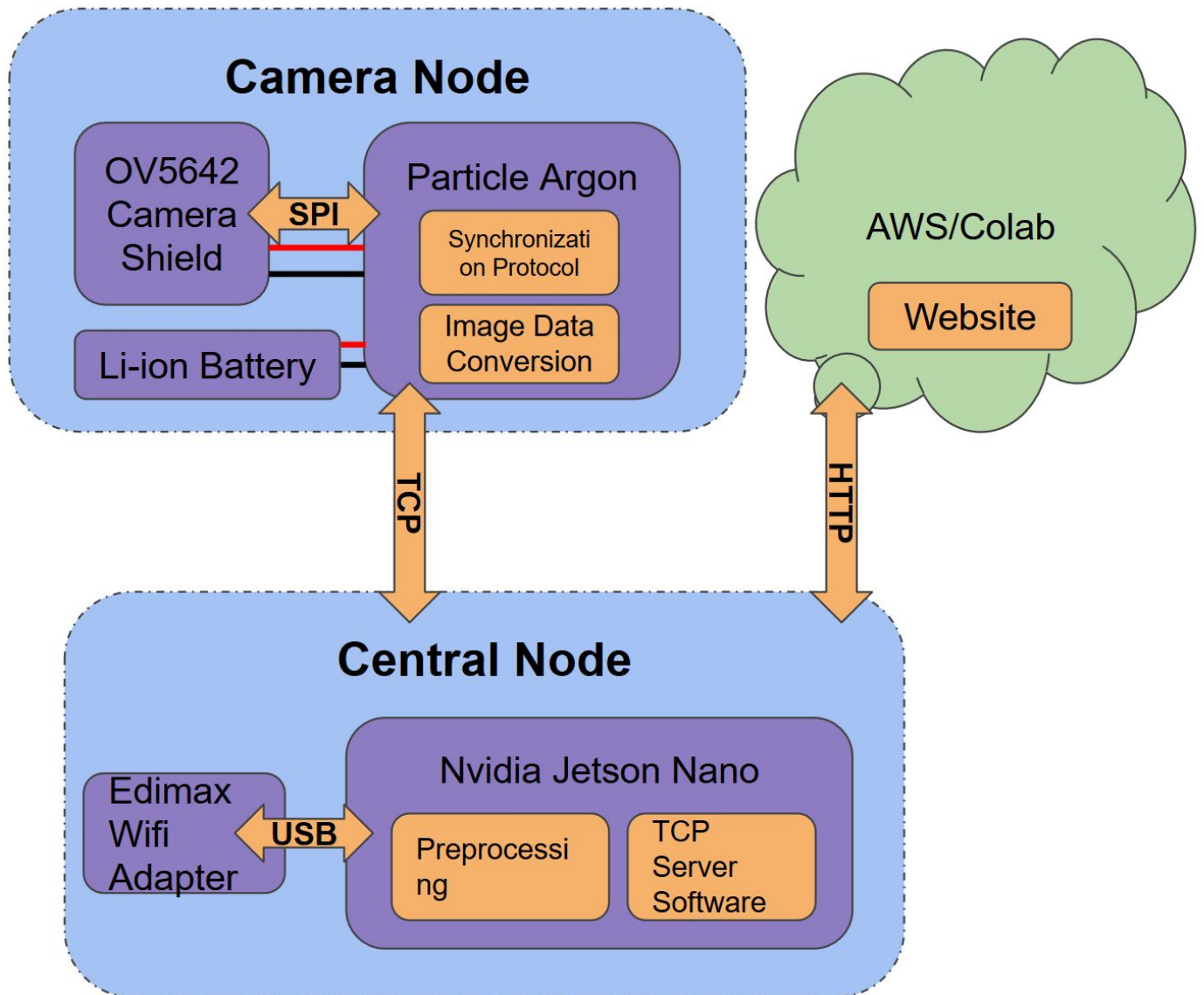
Fig. 1. Block Diagram of Node Network with 1 Camera Node
