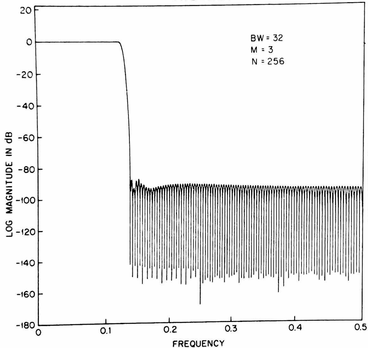
Fig. 3.31 Frequency response of a frequency sampling lowpass filter.
