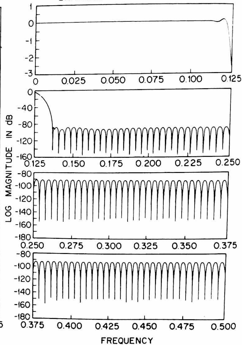
Fig. 3.31 Frequency response of a frequency sampling lowpass filter.
