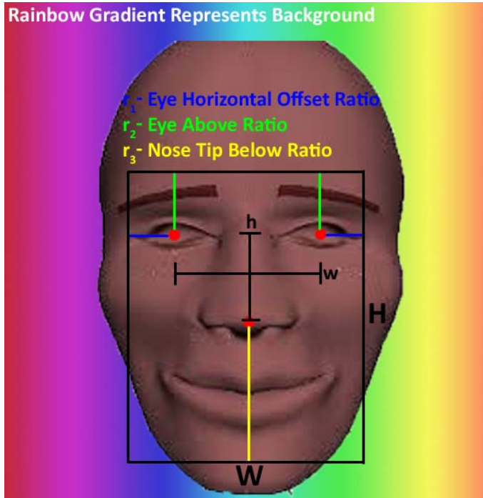
Figure 8: Landmark-fixing Normalization
