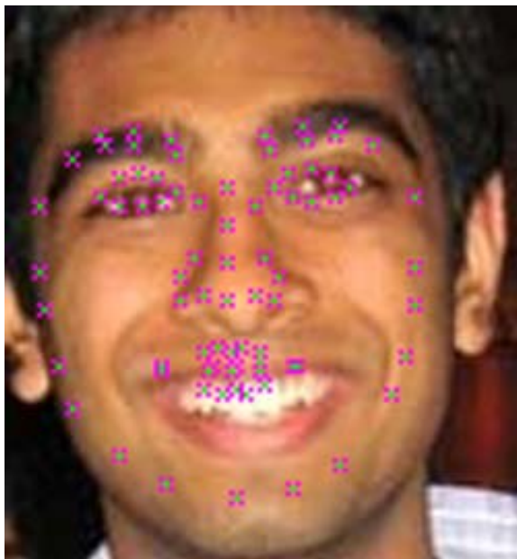
Figure 4: Incorrect Landmarks
