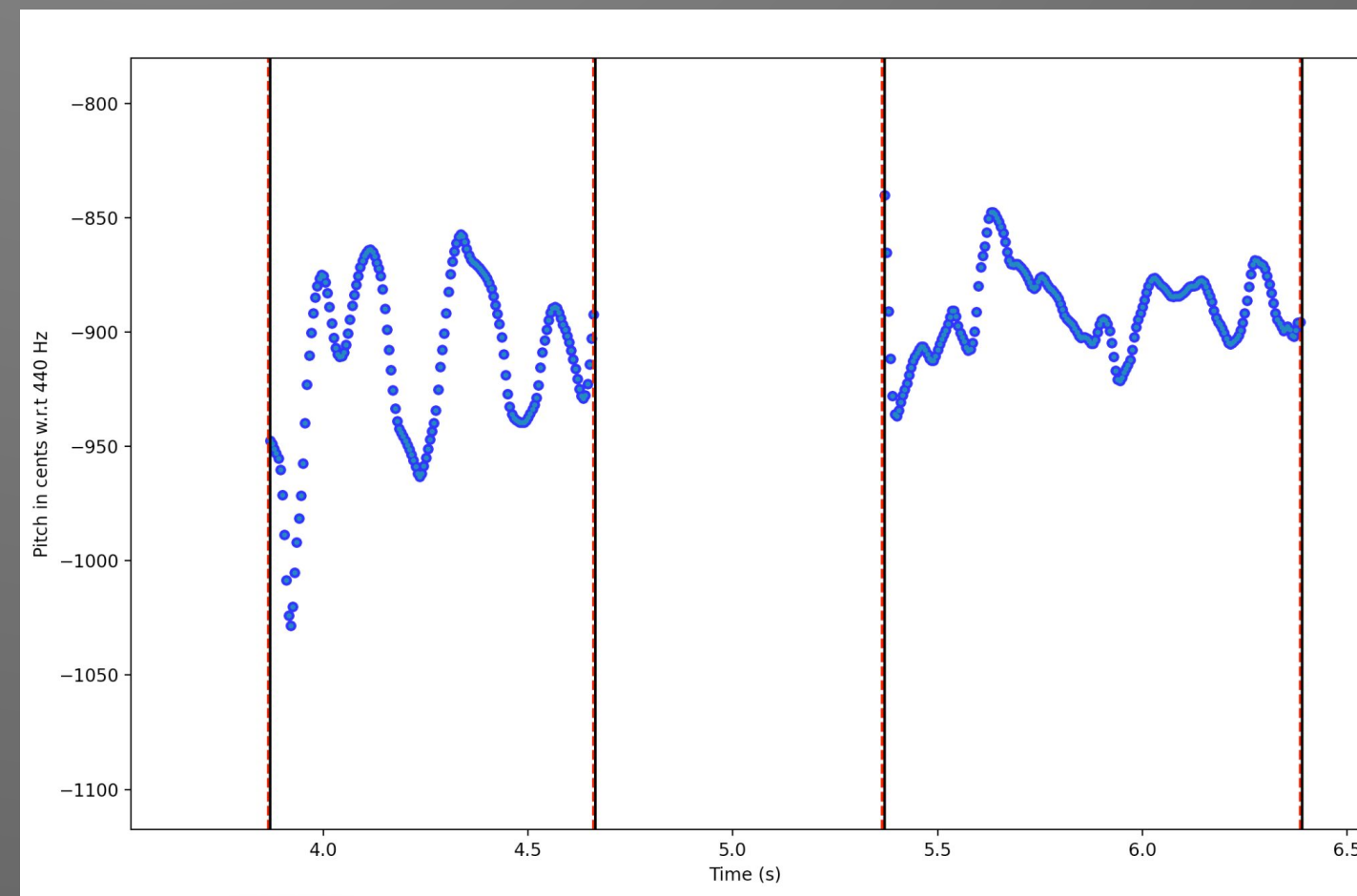
Algorithm used to segment pitch contours to musical notes
